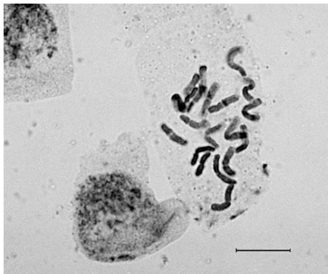
Fig. 7. Phlomis cypria subsp. occidentalis – root tip metaphase, showing 2n = 20 chromosomes. – Scale bar = 10 \mu\text{m} .
