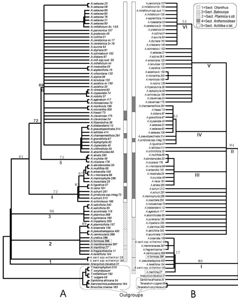
Fig.1. Strict consensus trees for Achillea s.l. (taxa from all sections) and related Anthemideae genera from nrITS data (A: tree length = 397, CI = 0.48, RI = 0.75) and cptrnL-F data (B: tree length 101, CI = 0.88, RI = 0.97) in juxtaposition. Bootstrap percentages (>50%) are shown above branches. Important clades are designated by arabic numerals below branches in A and by roman numerals in B. Taxa names with accession numbers correspond to Appendix 1 in Guo & al. (2004) and those listed in 'Material and methods'. Up-to-date assignment of taxa to Achillea sections is shown by two vertical reference bars in the middle, signatures are explained in the insert.
