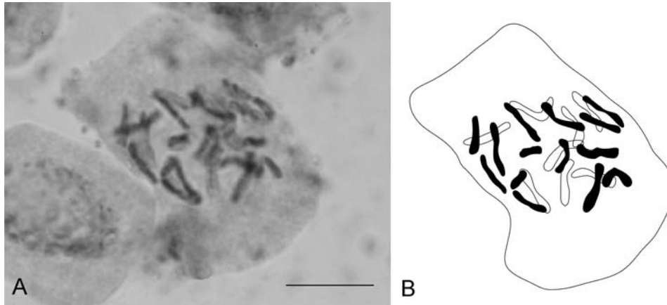
Fig. 3. Peucedanum isauricum , metaphases of root-tip mitoses, 2n = 22 (from Ulrich 3/28d). – Scale bar = 10 \mu\text{m} .
